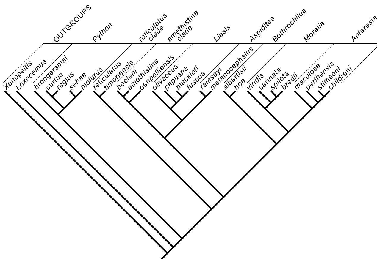
Figure 5. Pyron et al. 's (2013) phylogenetic hypothesis of the pythons based on a combined analysis of seven nuclear DNA loci and five mitochondrial DNA regions.
