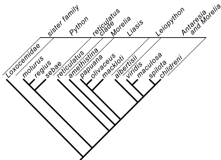
Figure 2. Lawson et al. 's (2004) phylogenetic hypothesis of the pythons based on sequence analysis of the mitochondrial cytochrome b region.
